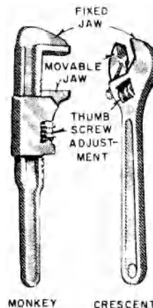
adjustable wrenches
