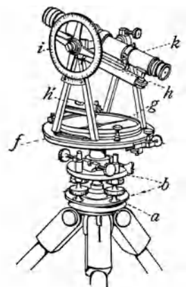
transit: a, tripod stand; b, leveling plates; f, vernier; g, compass; h, h', levels; i, vertical circle; k, telescope
