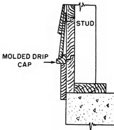
water table, 1
