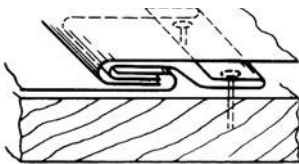
concealed cleat
