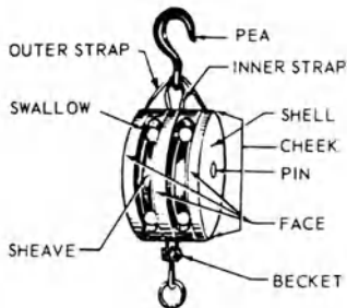
pulley block
