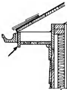
eaves fascia
