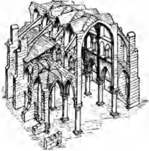
Gothic architecture showing construction of a Gothic church, illustrating principles of isolated supports and buttressing
