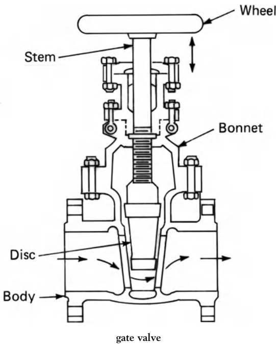
gate valve
