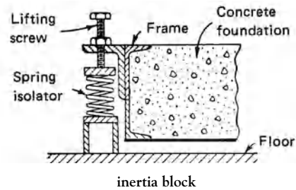
inertia block
