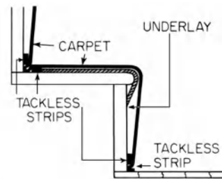
tackless strip
