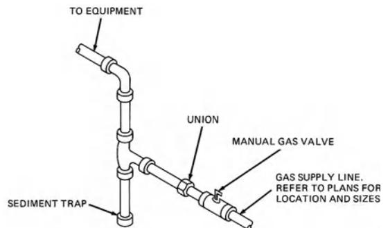
sediment trap, 2
