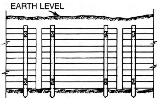
horizontal sheeting
