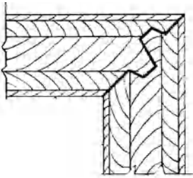
lock miter
