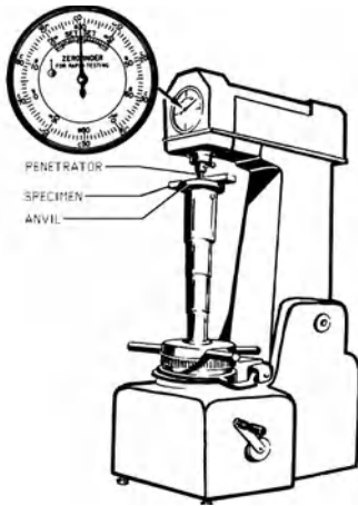
Rockwell hardness tester
