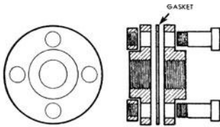
flange union
