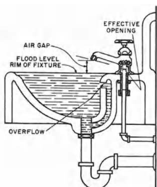
lavatory, 1
