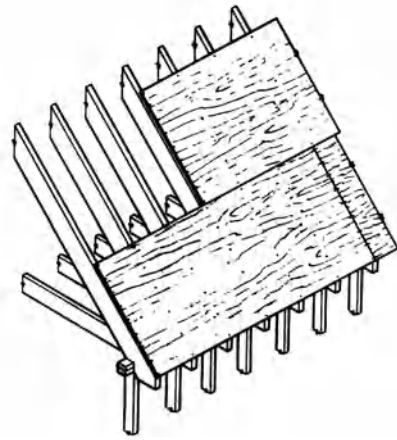
plywood roof sheathing
