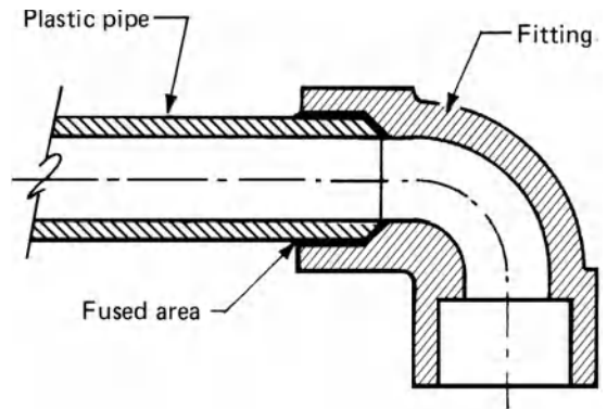
heat-fusion joint
