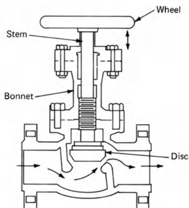
globe valve
