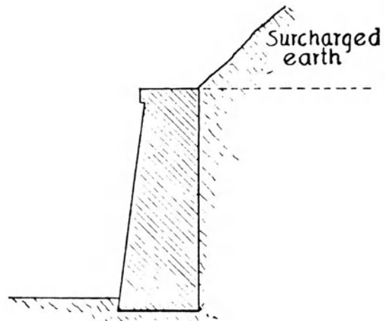
surcharged earth
