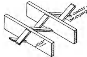
cross bridging
