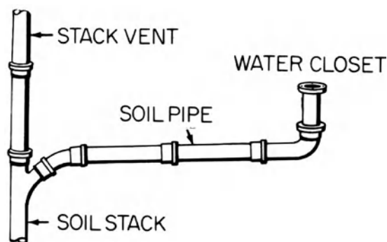
soil stack
