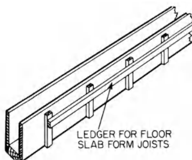
ledger, 1
