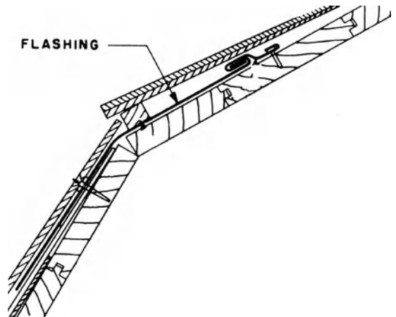
concealed flashing
