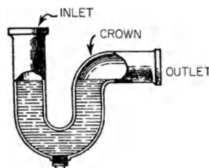
crown, 9
