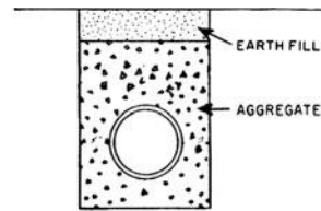
underdrain
