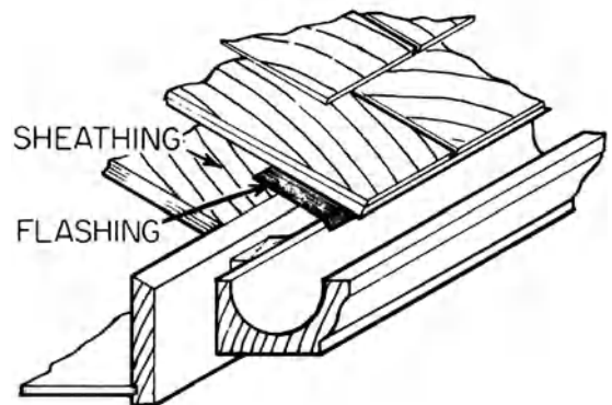
wood gutter
