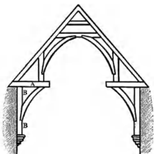
hammer beam: A
