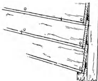
colonial siding
