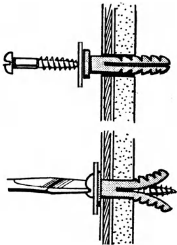
anchorage device
