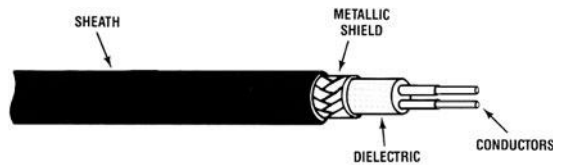
twin axial cable
