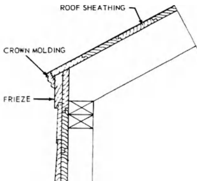
crown molding
