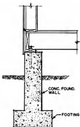
footing
