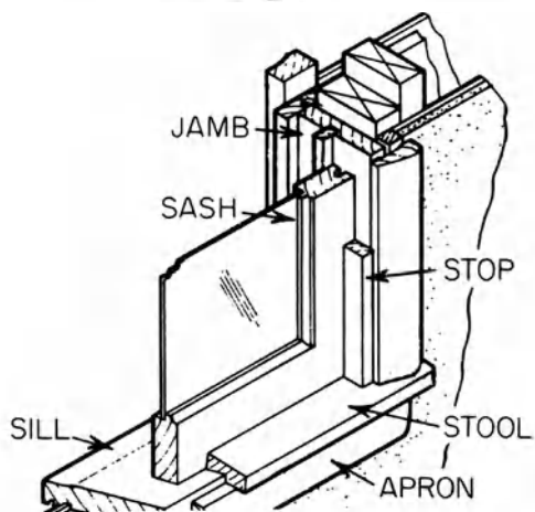
window: details
