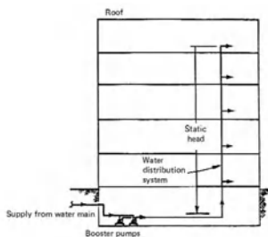
simplified diagram of a water distributor system employing a booster pump
