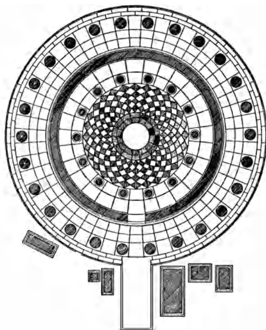
tholos, 1 at Epidaurus, plan
