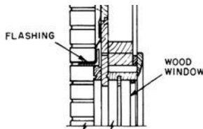
head flashing
