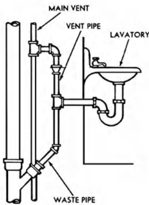
individual vent
