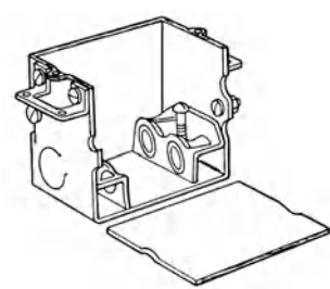
outlet box
