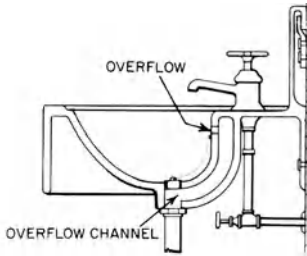
overflow, 1
