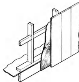
vertical siding
