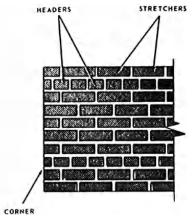
common bond
