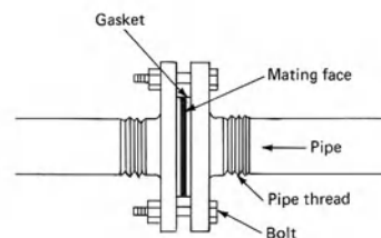
flanged joint
