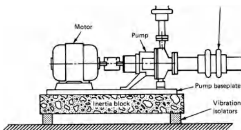
pump on an inertia block
