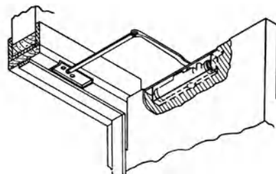
overhead concealed closer
