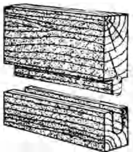
dressed and matched boards
