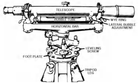
wye level
