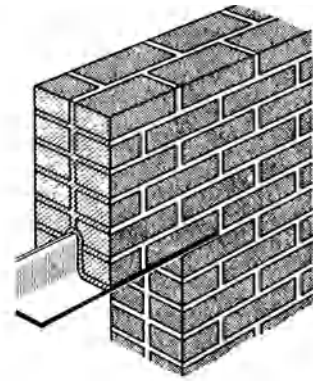
steel lintel
