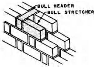
bull stretcher, 2 and bull header, 2
