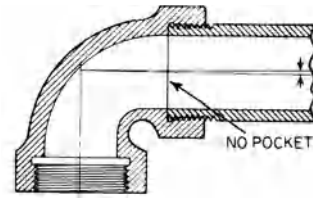
drainage fitting
