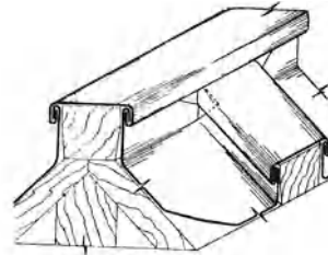
batten seam
