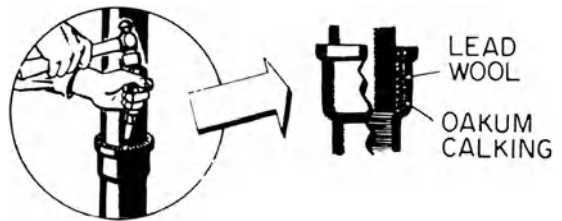
lead wool applied as caulking
