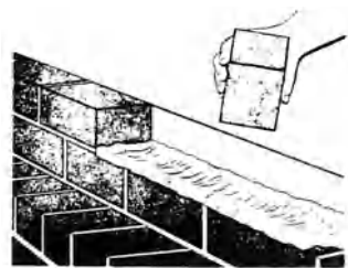
bed joint, 1
