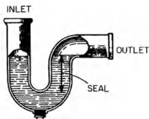
seal, 4
