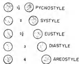
Diagram of intercolumniation
