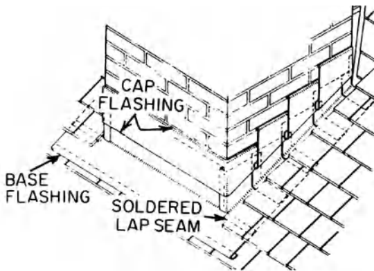
stepped flashing
