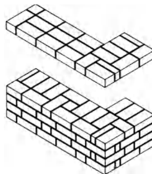
Flemish garden-wall bond
