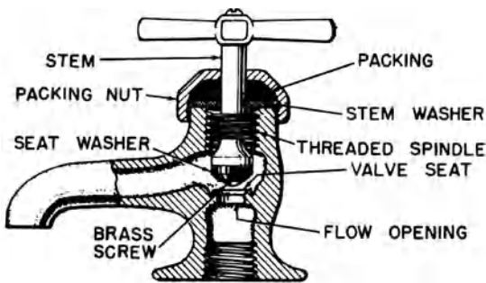
compression faucet
