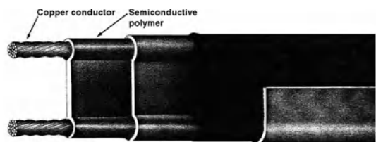
strip heater
