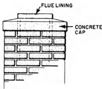
flue lining
