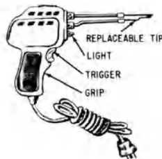
soldering gun
