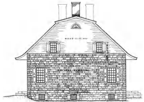
flared eaves
