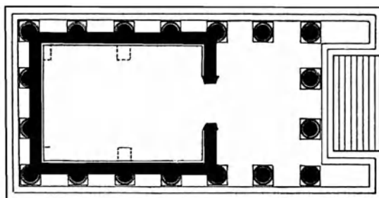
pseudoperipteral
