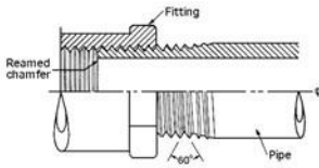
threaded joint
