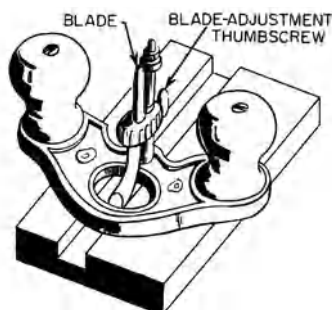
router plane
