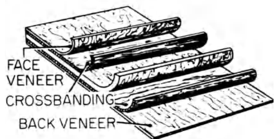
veneered plywood
