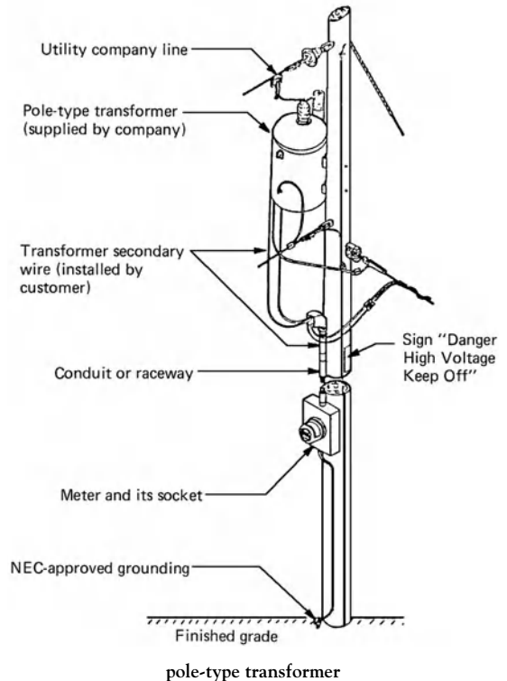
pole-type transformer
