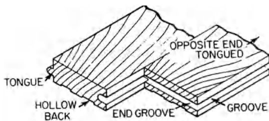
matchboards
