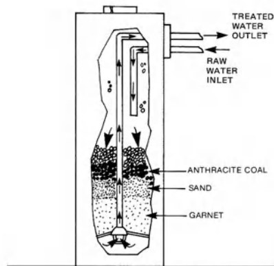
multimedia filter
