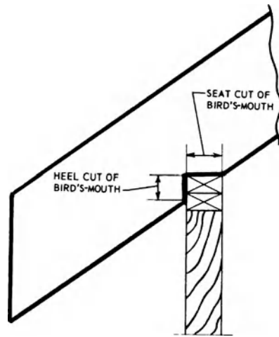
bird's-mouth, 1
