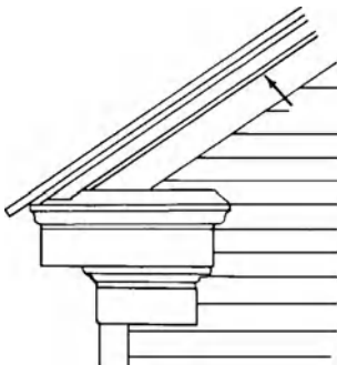
raking molding
