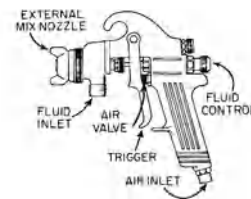
spray gun
