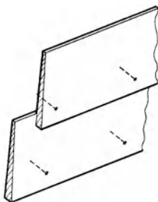
clapboard
