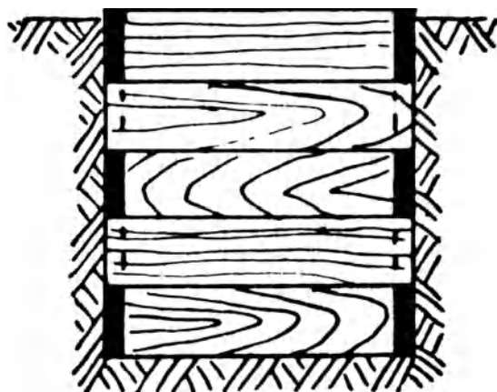
horizontal sheeting
