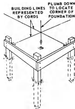
batter boards
