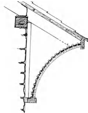
coved eave
