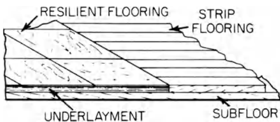
underlayment, 1
