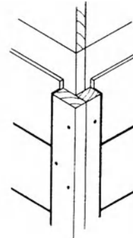
corner board
