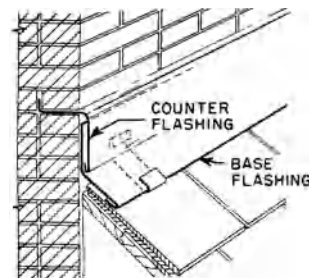
counterflashing
