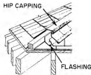
hip capping
