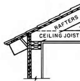
open cornice
