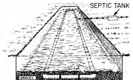
seepage bed
