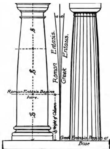
entasis: proportions are much exaggerated
