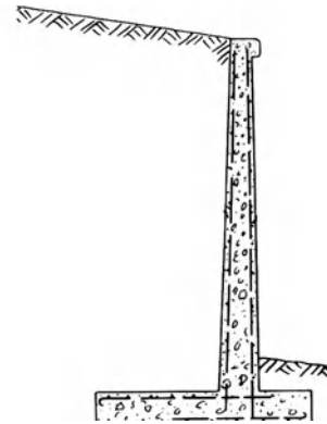
cantilever wall
