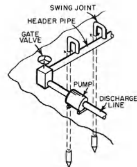
well-point system
