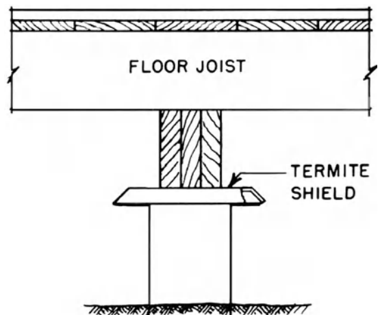
termite shield
