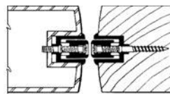
mortised astragal
