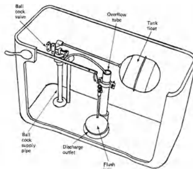
flush tank
