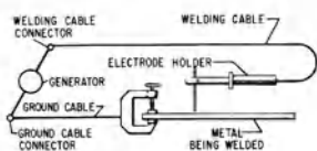
arc welding: above , with bare electrodes; below , circuit
