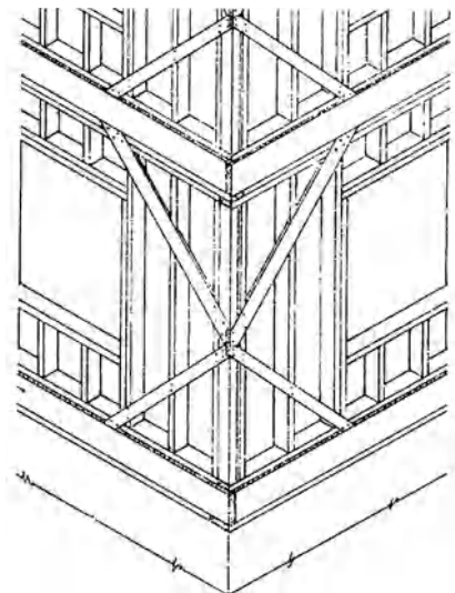
corner brace
