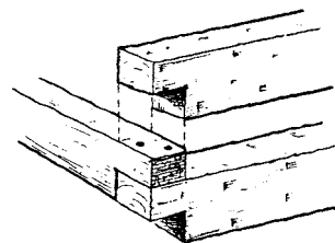
half-cut notch
