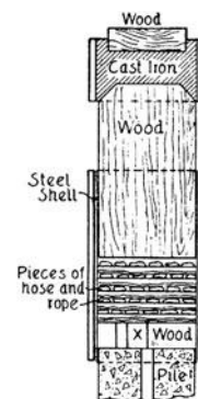
cushion head
