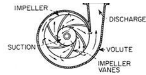
centrifugal pump
