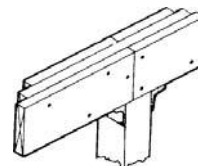
built-up beam on a post
