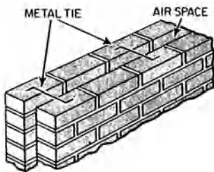
metal ties, 1
