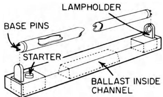
fluorescent lamp
