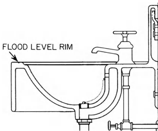
flood-level rim
