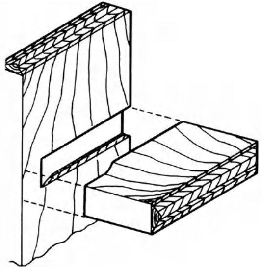
stopped dado
