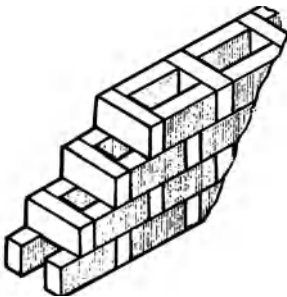
rowlock cavity wall
