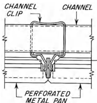
channel clip, 1
