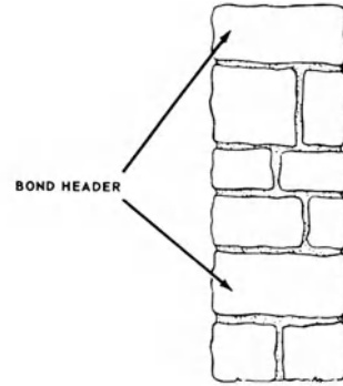
bond header
