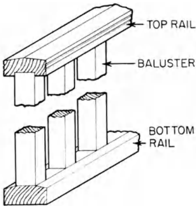
balustrade
