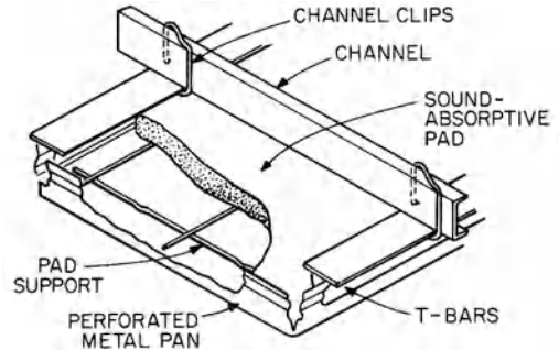
perforated metal pan
