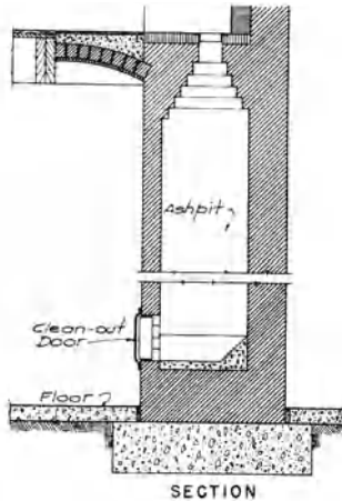
ashpit
