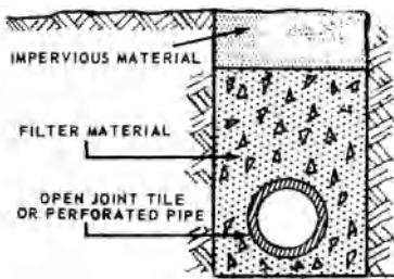
absorption trench
