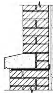
sill course
