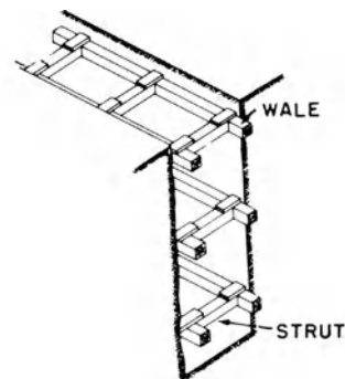
open sheeting
