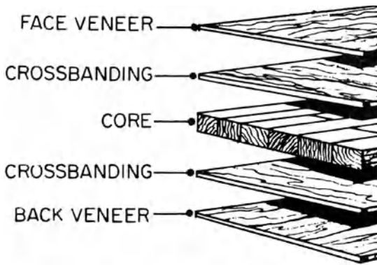
crossbanding, 1
