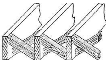
herringbone bridging
