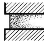
recessed pointing
