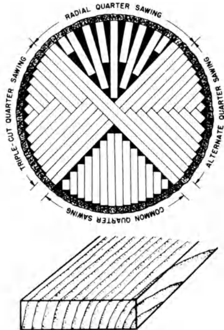
quartersawn
