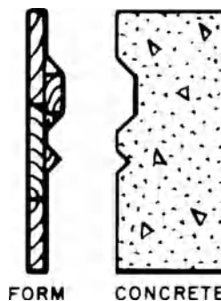
mold for finishing concrete
