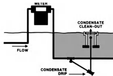
drip, 4
