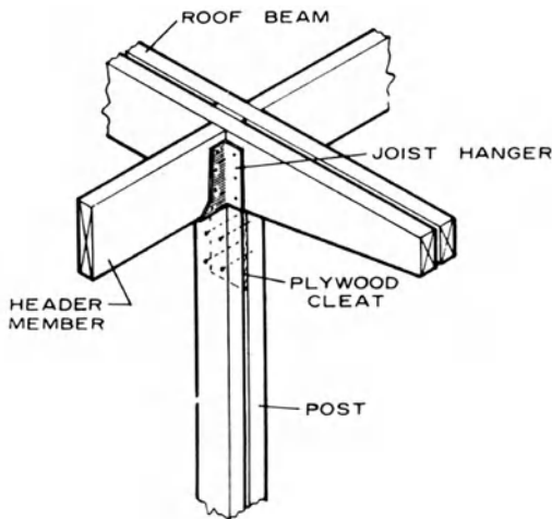
post-and-beam framing
