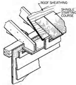
starting course
