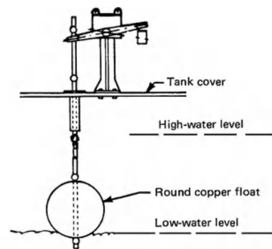
float switch in a water tank
