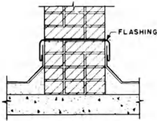
through-wall flashing
