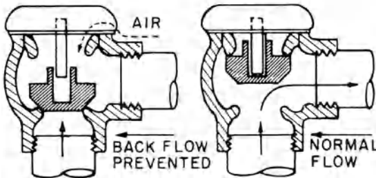
vacuum breaker
