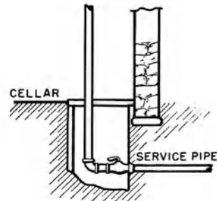
service pipe
