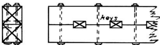
keyed beam
