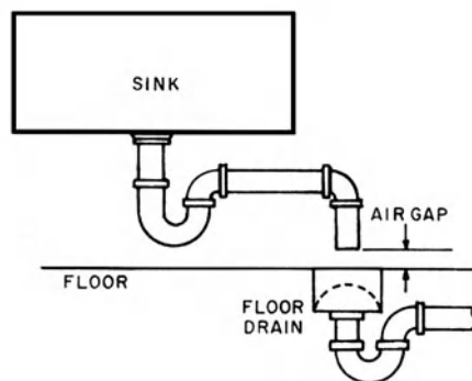
indirect waste pipe
