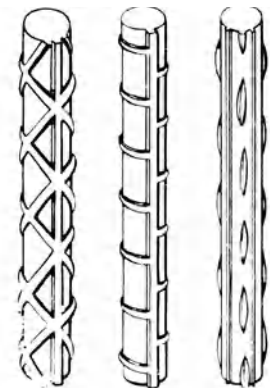
deformed bars
