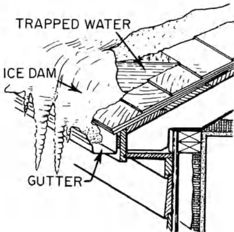
ice dam
