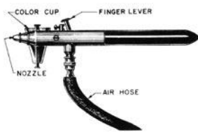
airbrush
