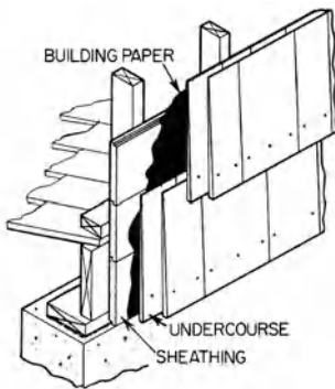
undercourse
