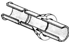
bell-and-spigot joint
