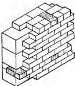
masonry ties, 1
