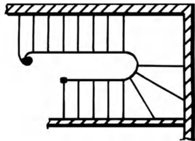
geometrical stair
