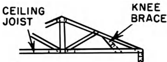
knee brace
