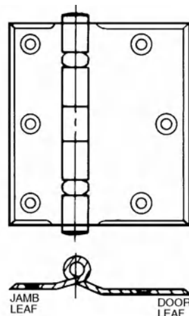
full-surface hinge
