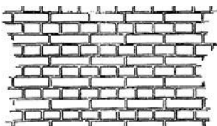
English bond
