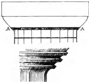
annulets: A, of a Doric capital. Shown enlarged in lower figure
