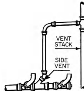
side vent
