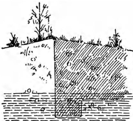
groundwater
