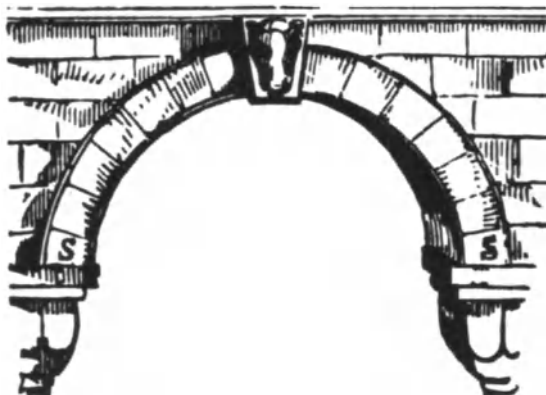
springer, 1: S
