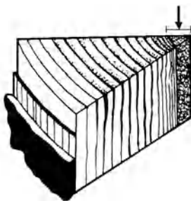
pith
