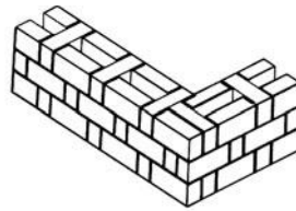
rat-trap bond
