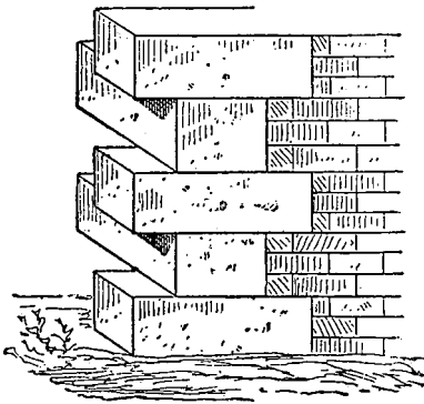
in-and-out bond
