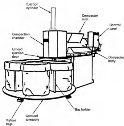
carousel packer
