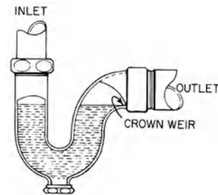
crown weir
