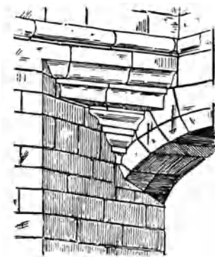
skew arch
