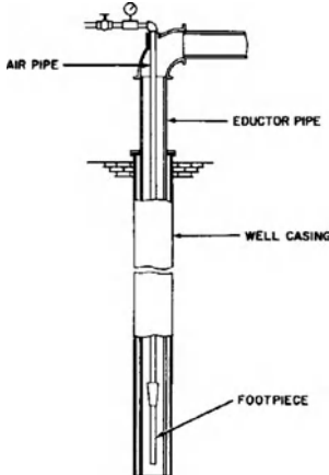
air-lift pump
