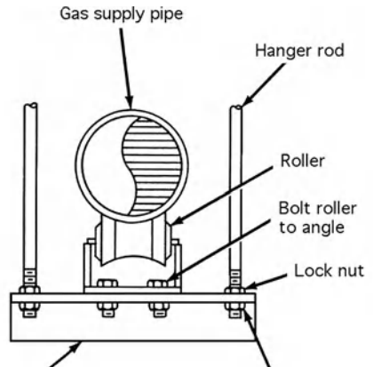
trapeze hanger with roller support
