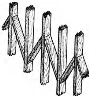
diagonal bridging, 2
