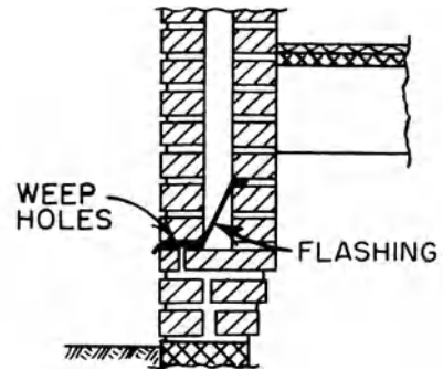
cavity flashing
