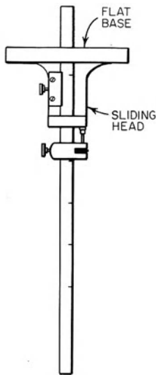
depth gauge
