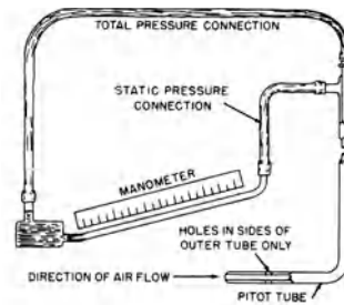
pitot tube
