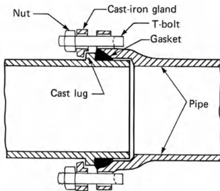
typical mechanical joint
