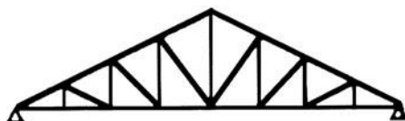
Howe truss
