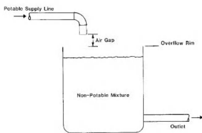
air gap, 1
