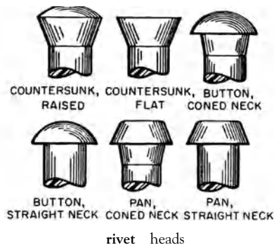
rivet heads
