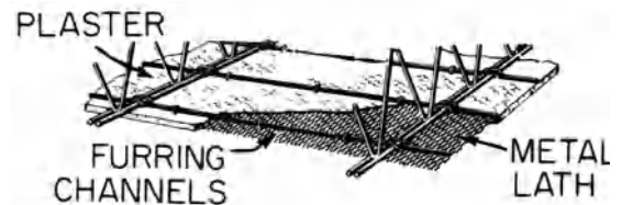
furring
