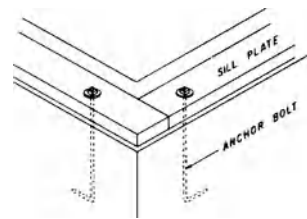
anchor bolt
