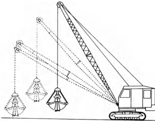
clamshell, 2
