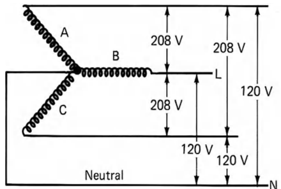
wye connection, 1
