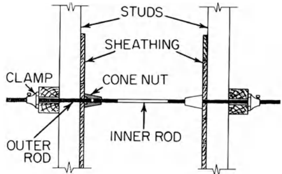
cone-nut tie
