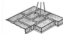
three-quarter closer
