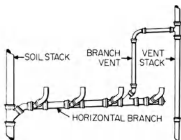
branch vent, 1
