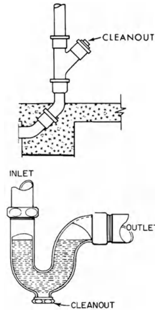
cleanout, 1: above: for cleaning pipe run; below: for a P-trap
