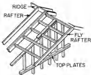
fly rafter
