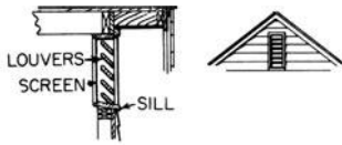
outlet ventilator
