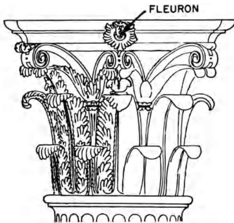
fleurion, 1
